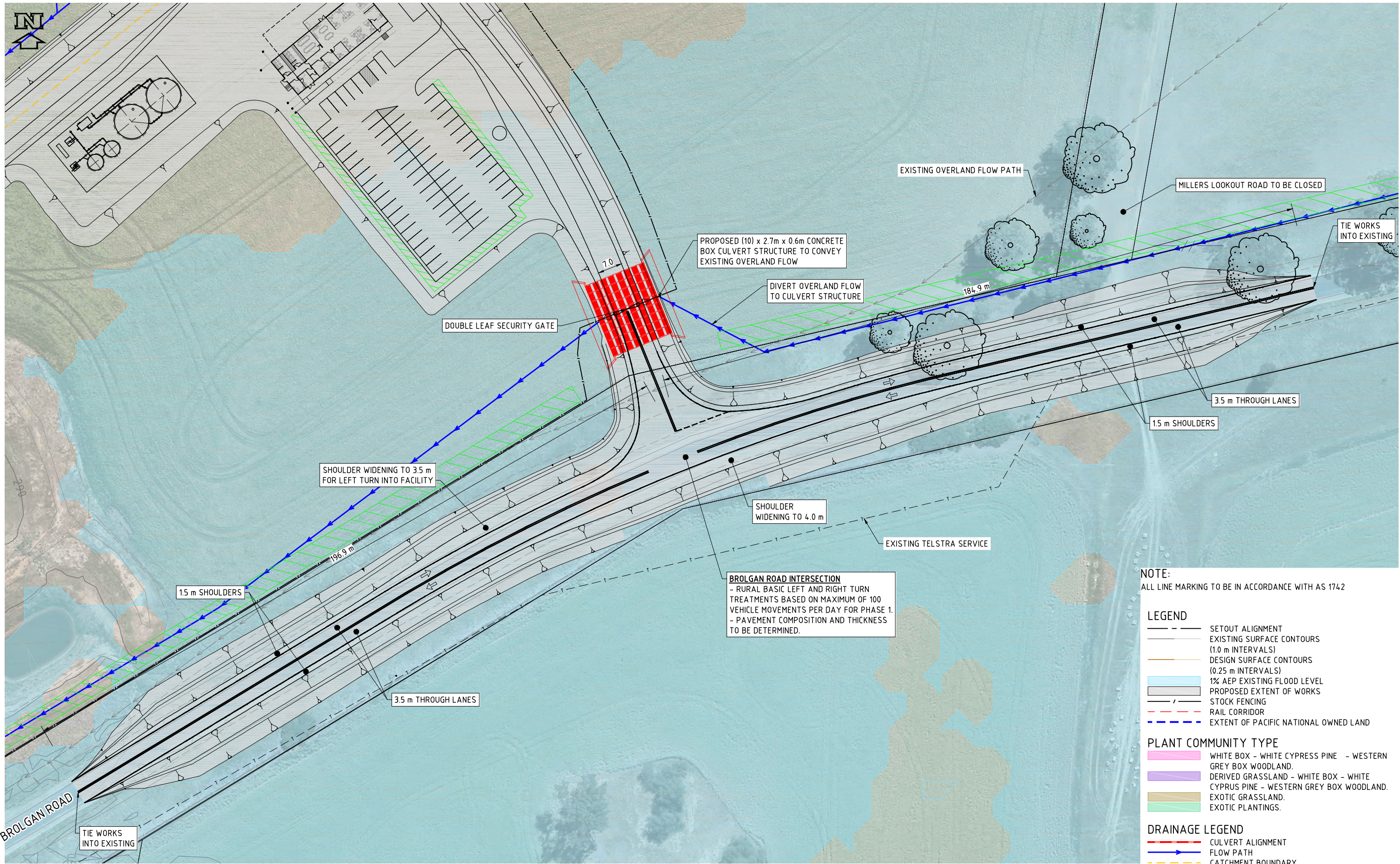
BROLGAN ROAD INTERSECTION SCALE 1:500
